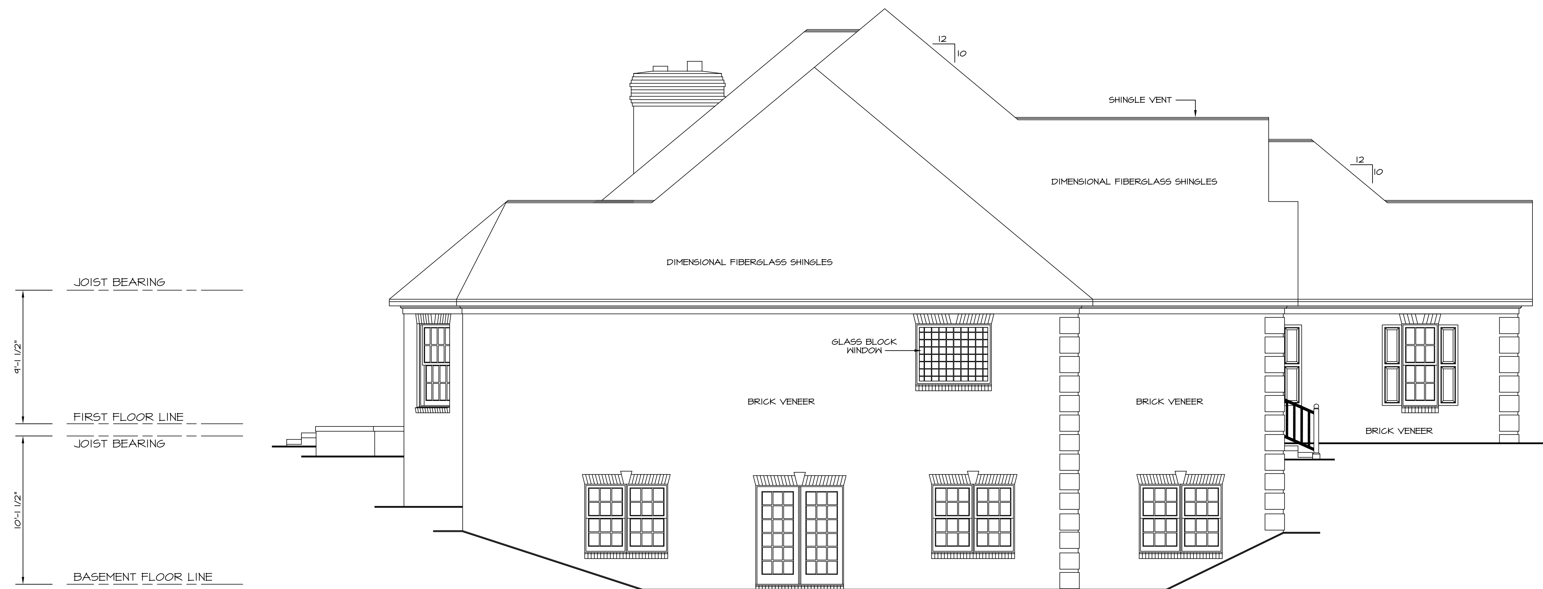
LEFT SIDE ELEVATION
